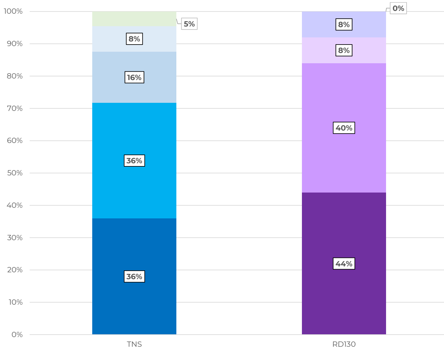
Figure 23: Recommend (n=25)
