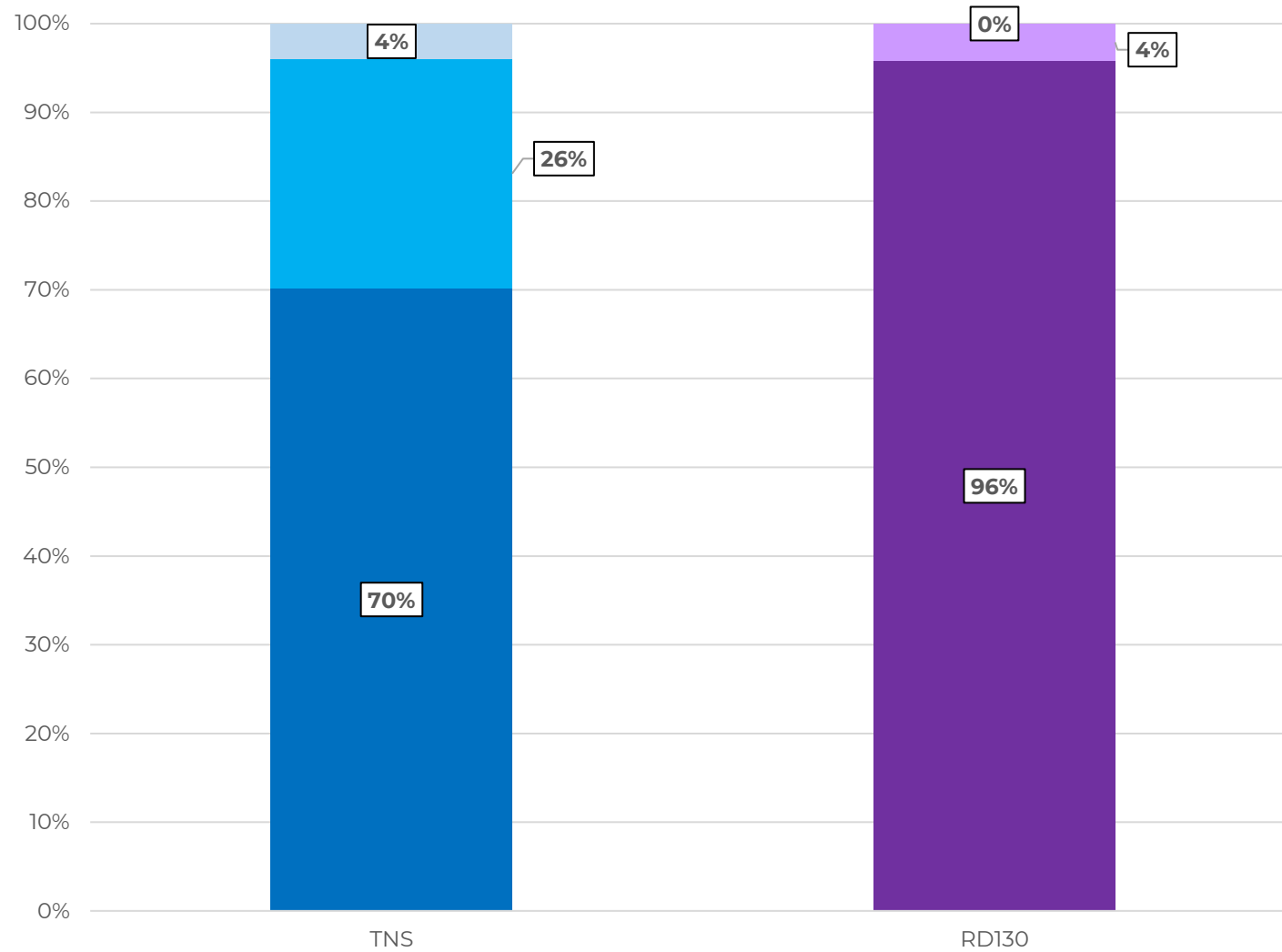
Figure 18: Respect (n=24)
