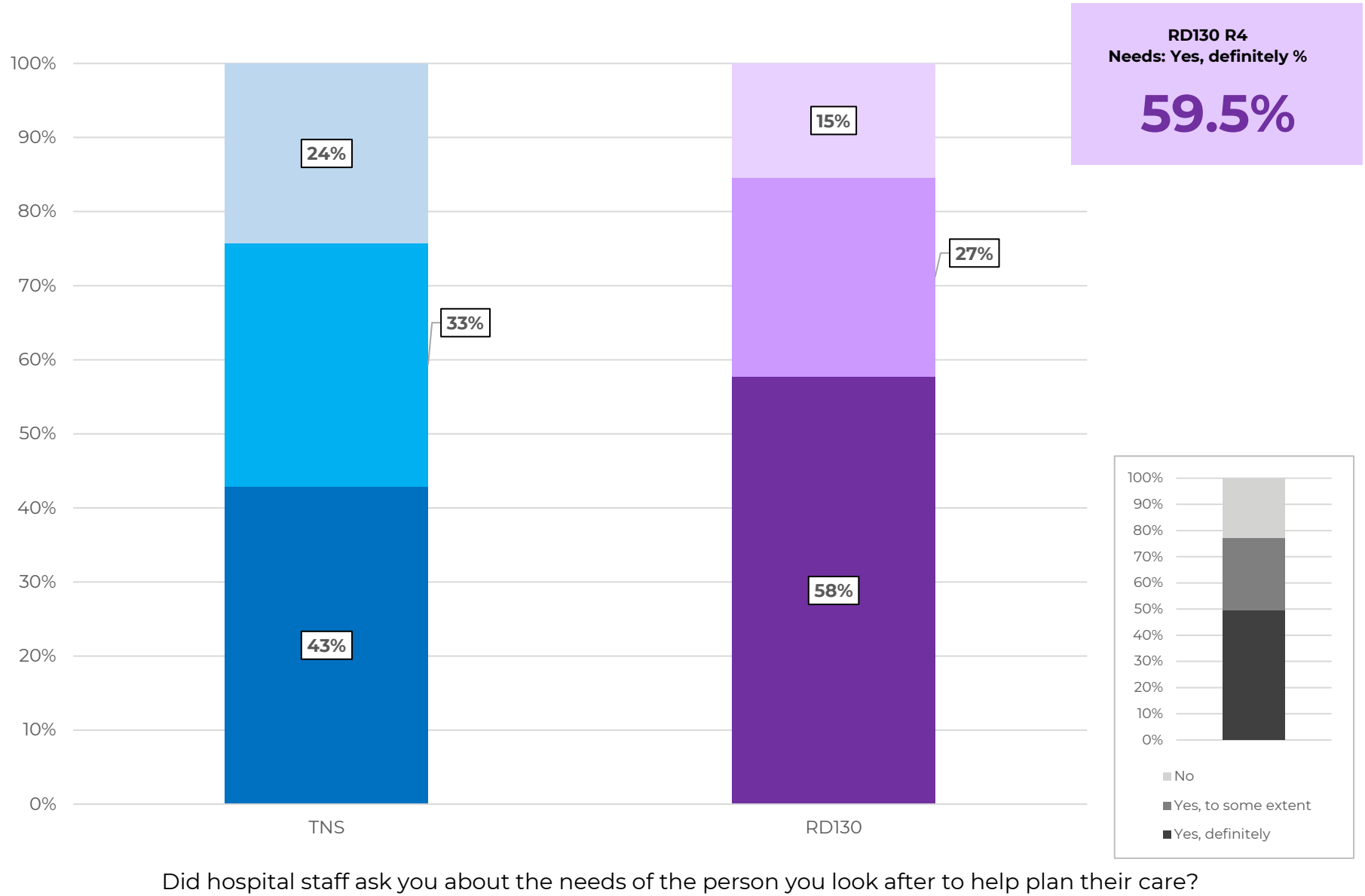
Figure 21: Needs (n=26)
